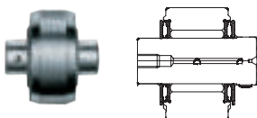
Cylindrical rollers roller version for standard inserts
