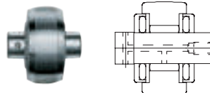
Convex rollers for conical workpieces and for following steady rest arrangement
